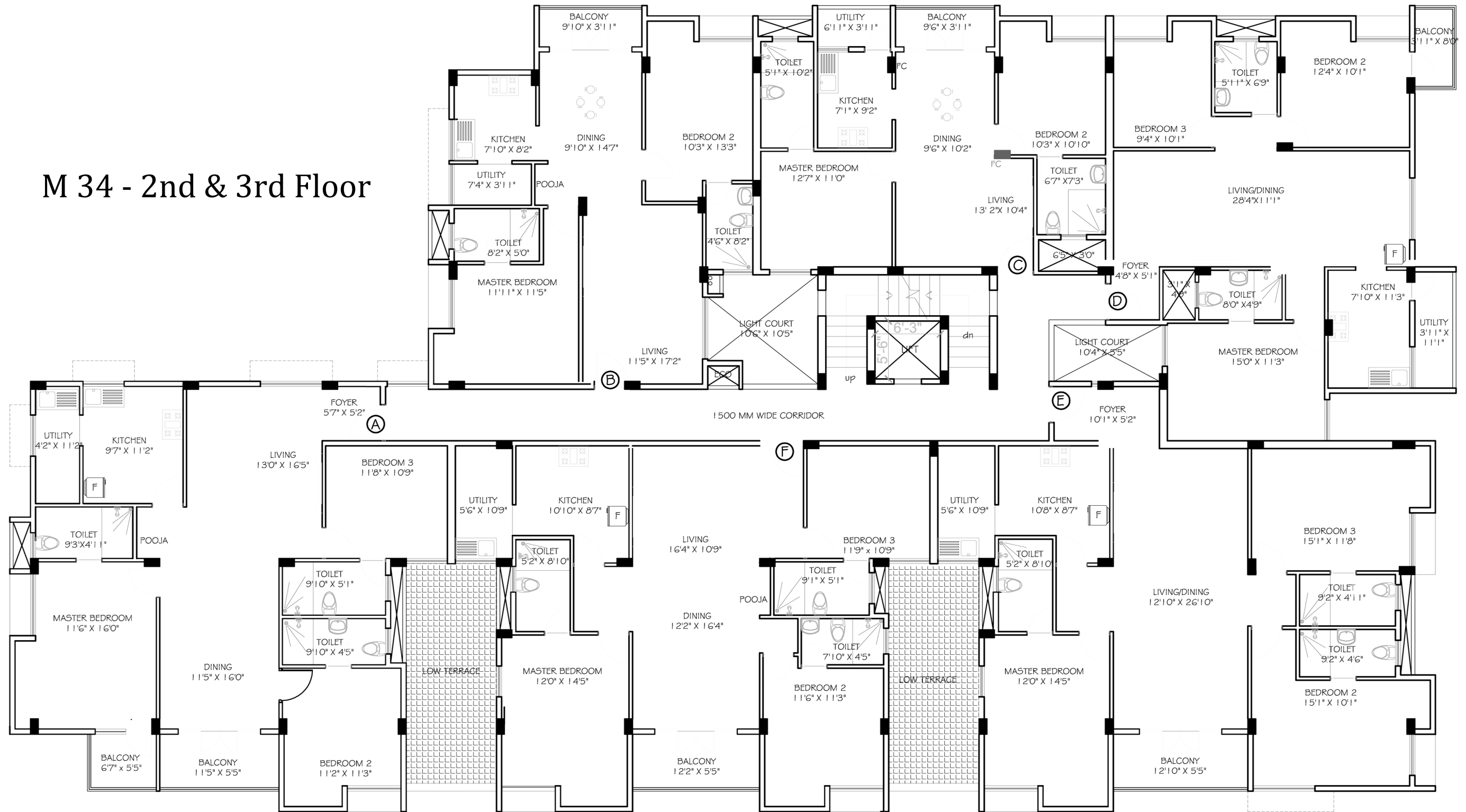
TYPICAL FLOOR PLAN (SECOND & THIRD FLOOR)
